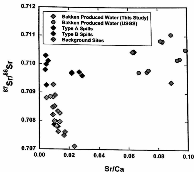
Figure 3. ^{87}\text{Sr}/^{86}\text{Sr} vs \text{Sr}/\text{Ca} (mass) ratios in Bakken produced waters, spill waters, and background waters. Note the large Sr isotopic and Sr/Ca ratio differences between the Bakken brines and background surface water in the study area. The ^{87}\text{Sr}/^{86}\text{Sr} ratio of the highly mineralized background water decreases with Sr/Ca, indicating a Sr source with a conspicuously lower ^{87}\text{Sr}/^{86}\text{Sr} signature as opposed to the relatively high ^{87}\text{Sr}/^{86}\text{Sr} ratios of the Bakken brines and spill waters. This distinction verifies that both type A and type B spill waters originated from the Bakken oil and gas wastewater.
